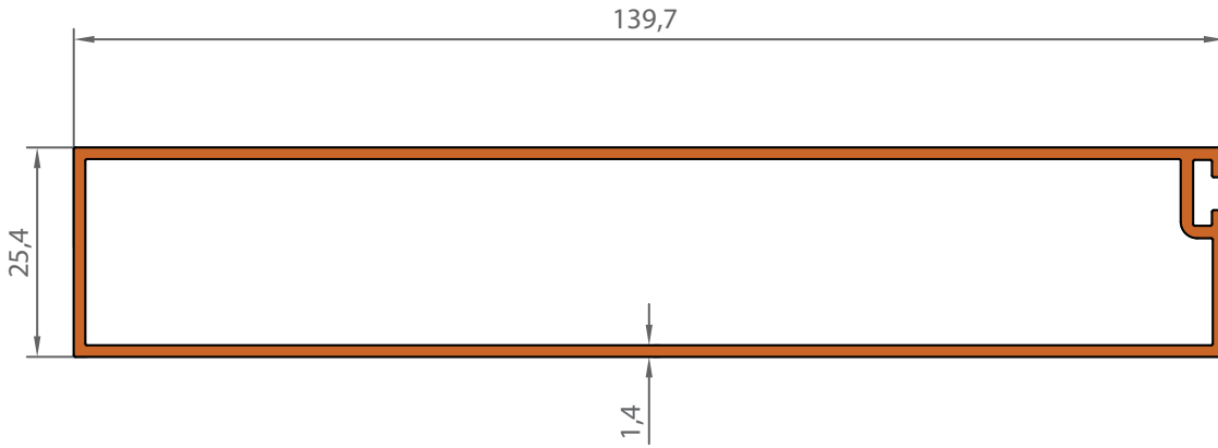
1006 1,266 KG/M
