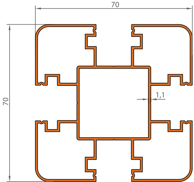
1220 1,515 KG/M
