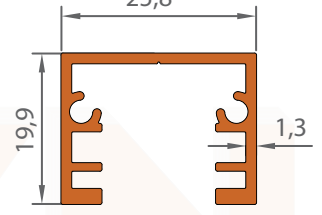
1220 1,515 KG/M
