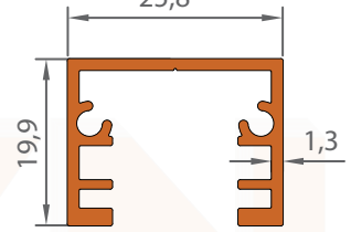
1220 1,515 KG/M
