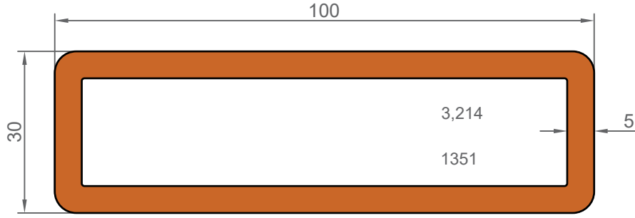
1351 3,214 KG/M
