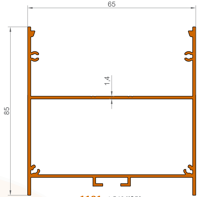
1101 1,548 KG/M
